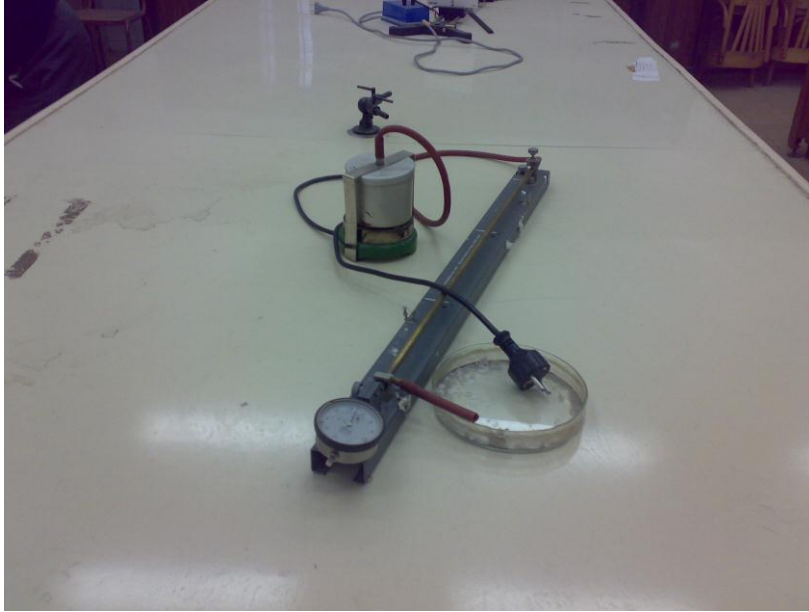
Experiment of determining linear thermal expansion coefficient
